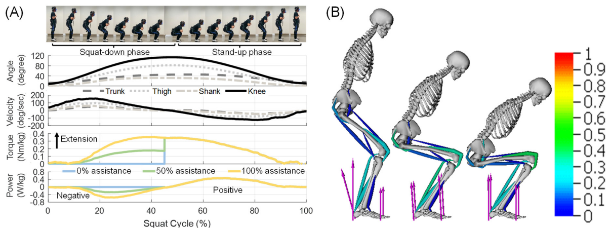
Fig. 5: Computational musculoskeletal biomechanics model driven by experimental data. (A) The mean of measured knee angle and velocity profiles averaged from all conditions and assistance torque and power profiles of a representative subject for each control strategy. (B) Predicted muscle activations during the squat-down phase. The color of the muscles indicates their activation, as shown in the color legend on the right. The arrows represent predicted ground reaction forces at the contact points.
