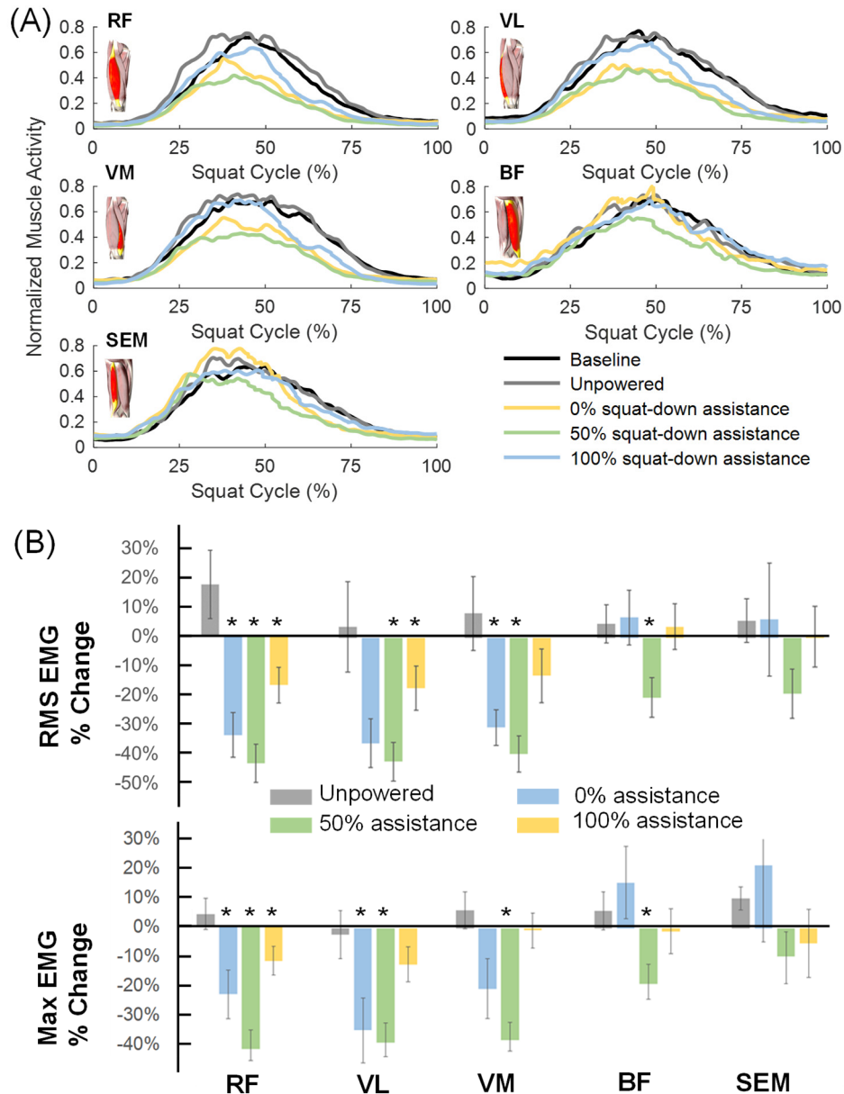
Fig. 7: Muscle strain mitigation results in terms of EMG. (A) Averaged activity of three extensors (RF, VL, VM) and two flexor (BF, SEM) muscles under different test conditions (baseline, unpowered, 0% squat-down assistance, 50% squat-down assistance, 100% squat-down assistance) across all subjects ( n = 7 ). The results showed that the exoskeleton with all three assistance strategies effectively reduced the activities of the three extensor muscles. (B) Changes in normalized RMS and Max EMG averaged across five squat cycles and all the subjects ( n = 7 ) in assisted and non-assisted conditions compared to baseline. The results showed that exoskeleton with moderate (50% assistance) level torque assistance strategies effectively reduced the activities of both extensor (RMS reduction of 39.39%-43.22%) and flexor (RMS reduction of 18.89%-20.25%) muscles.
