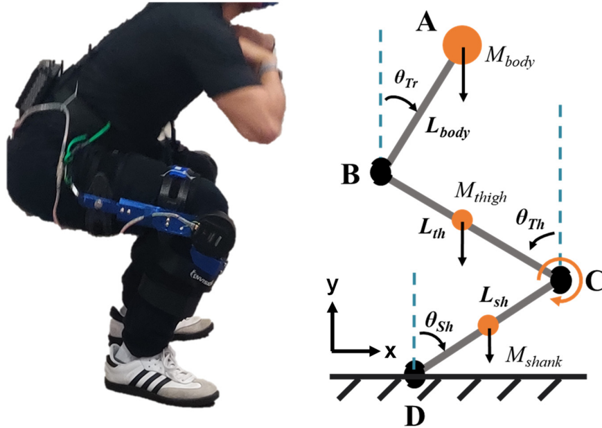
Fig. 3. The analytical biomechanical model for squatting. The annotations denote the combined mass of the upper body ( M_{body} ), the mass of the thigh ( M_{th} ), the mass of shank ( M_{sh} ), the length between the center of mass of M_b and the hip pivot ( L_b ), the length of the thigh between the hip pivot and knee pivot ( L_{th} ), the length of the calf between the knee pivot and angle pivot ( L_{sh} ), the trunk angle ( \theta_{Tr} ), the thigh angle ( \theta_{Th} ), and the shank angle ( \theta_{Sh} ).
