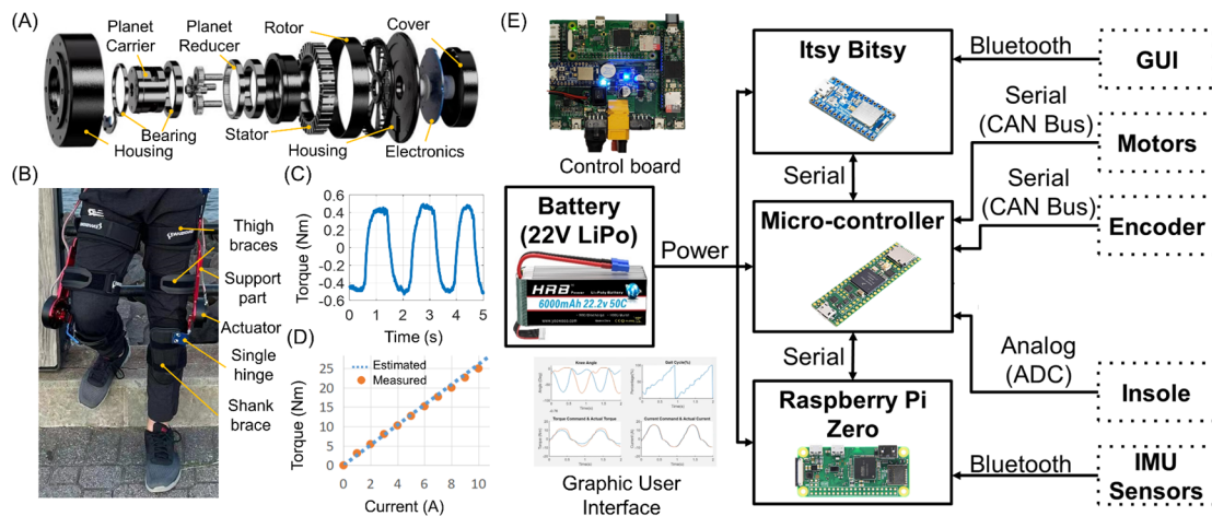
Fig. 2: Mechatronic design of the knee exoskeleton for squatting. (A) Customized quasi-direct drive actuator. (B) Portable knee exoskeleton. (C) Measurement of resistive torque. (D) Measured torque values (dots) alongside the theoretical values derived from the torque constant of the motor (dashed line). (E) Overall electronics schematic.
