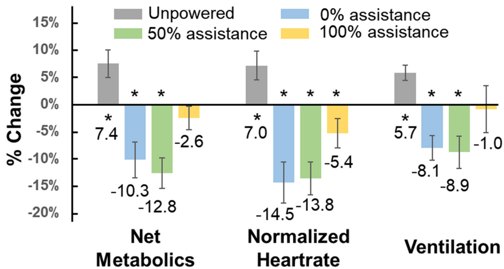
Fig. 6: Efficiency enhancement results in terms of metabolic cost, heart rate, and breathing ventilation. Average changes in net metabolic cost, normalized heart rate, and ventilation in assisted and non-assisted conditions compared to baseline conditions across all subjects ( n = 7 ). For every assistance condition, all three metrics were lower than the baseline condition, demonstrating the efficiency enhancement of the knee exoskeleton for squatting.
