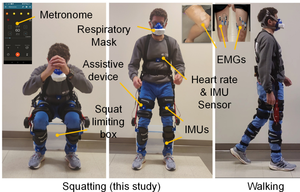
Fig. 1: A simple and generalizable controller for portable knee exoskeletons for squatting assistance aiming to reduce muscle activity (flexors and extensors EMG reduction), enhance user efficiency (metabolic cost, heart rate, and breathing ventilation reduction), or reduce perceived exertion (Borg 6-20 Scale and user preference reduction). The lightweight and portable knee exoskeleton can assist with squatting tasks without restricting walking kinematics.
